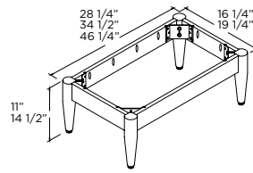
Vanity Leg Base 11" or 14-1/2"H 18" or 21"D VLBA30 VLBA30T VLBA36 VLBA36T VLBA48 VLBA48T
